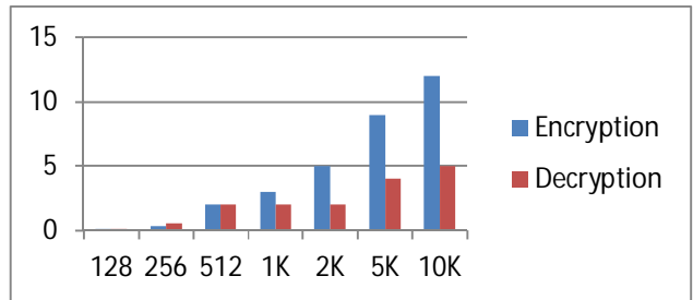
Fig 1: Performance on encryption and decryption timings of NTRU
