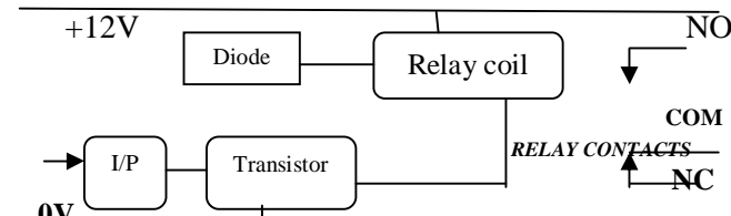
Fig 5 Drive circuit and protection diodes for relays
