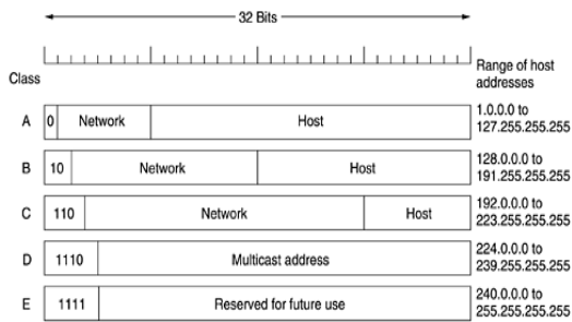
Fig 2. IP address
