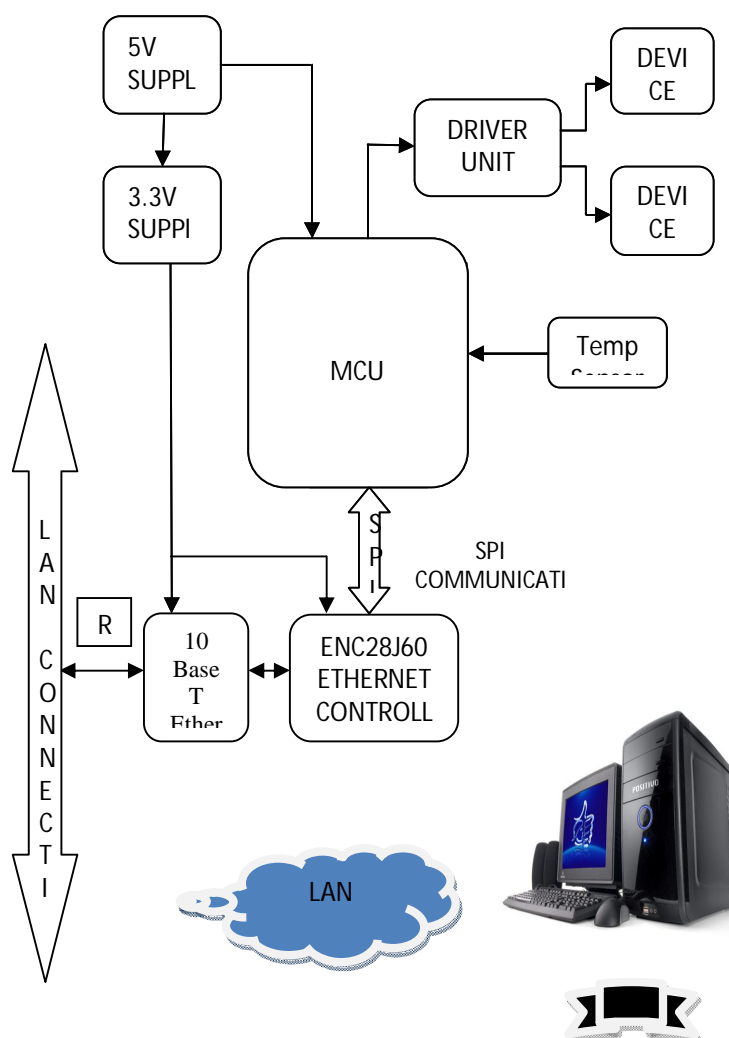
Figure 1. Module wise Block Diagram
