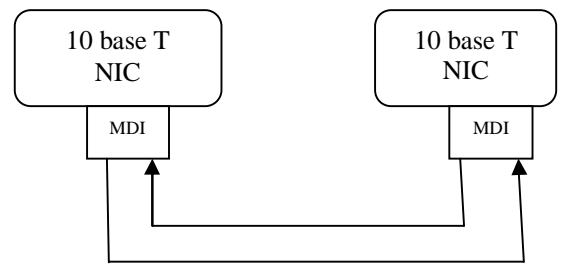
Four -pair category 3 or 5 UTP cable
