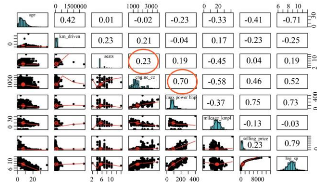
Fig. 7 Correlation matrix
