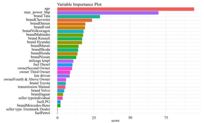
Fig. 13 Variable importance plot
