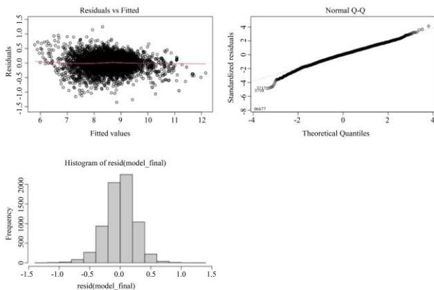
Fig. 12 Residual analysis
