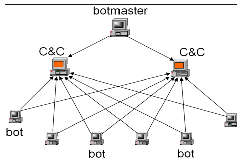
Fig.3 IRC Botnet
