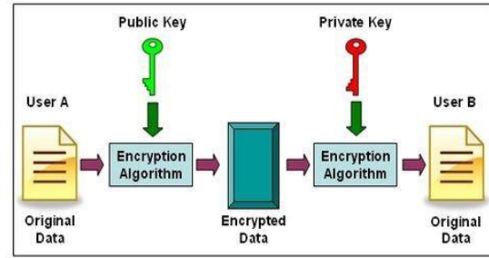
Fig 3 : Cryptography
